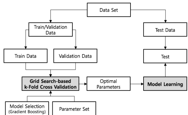
Fig. 2. Flow Chart of Model's Learning & Testing Procedure
